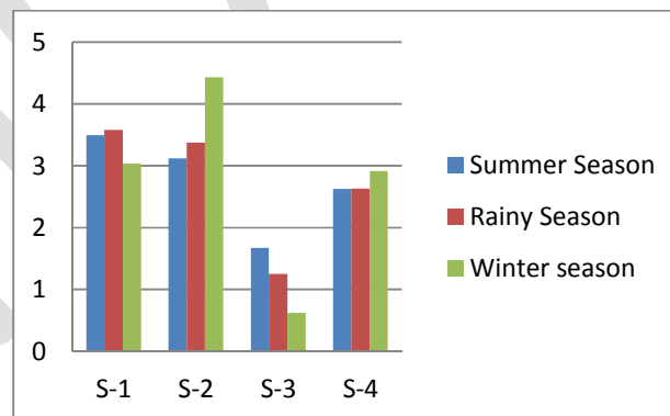
Figure 3. Margalef's Index of Species Richness of butterflies in different seasons
